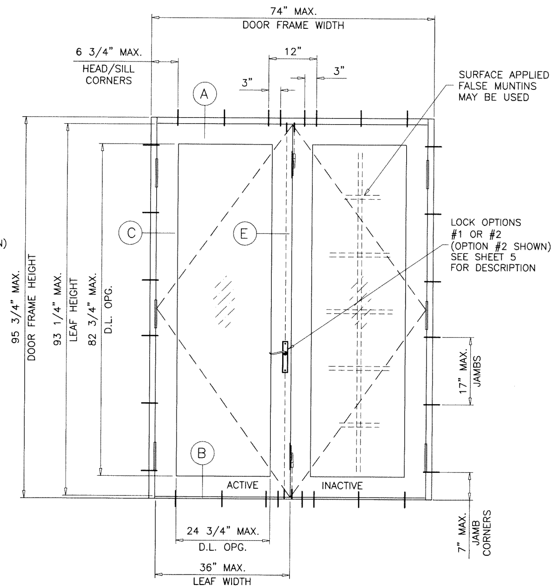
TYPICAL ELEVATION ( XX ) DUAL LEAF DOOR
