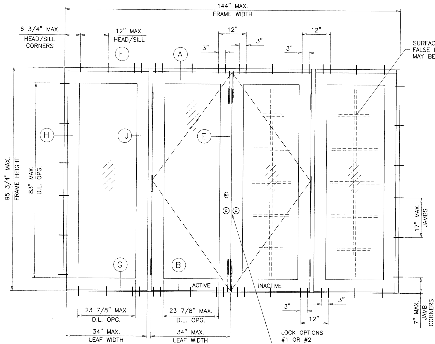
TYPICAL ELEVATION ( OXXO )
