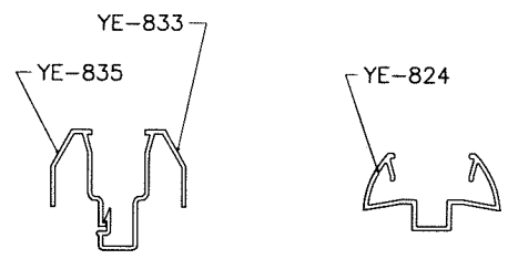
GLAZING ADAPTER OPTIONS
