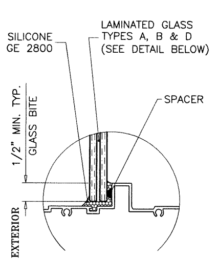
GLAZING DETAIL AT DIRECT SET SIDELITE
